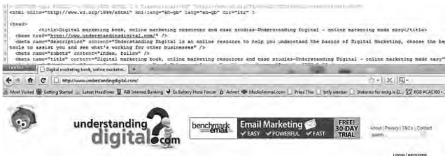
FIGURE 5.1 Screenshot showing title tag and meta-description as they appear in HTML source code, and the same page as it is rendered in the Firefox browser, showing the start of the same title tag in the active tab
